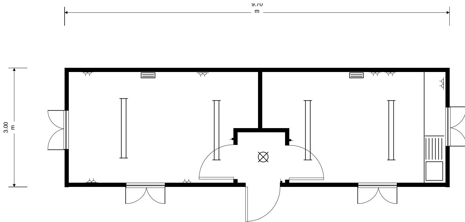
Suggested Layout New Build flat sided steel 32'x10' office canteen
